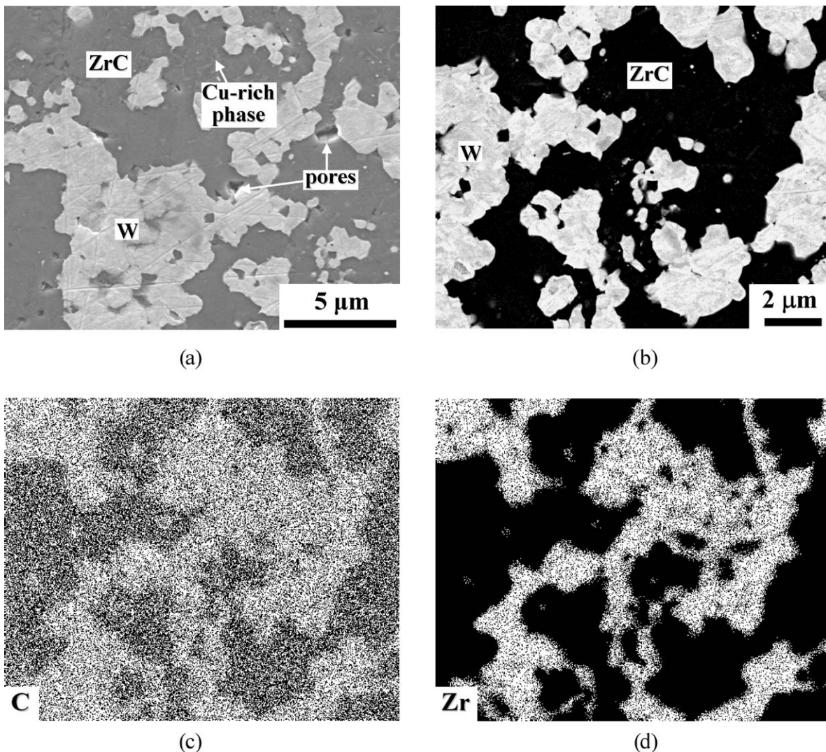
Figure 2 (a) Secondary electron and (b) backscattered electron images of composite specimens fabricated by the reactive infiltration of Zr_2Cu(l) into porous WC preforms (52.0 vol% porosity) at 1300°C. (c) C and (d) Zr X-ray maps associated with the backscattered electron image in (b). (e) W X-ray map associated with the backscattered electron image in (b). (f) Higher magnification secondary electron image of the Cu-rich phase in (a). (g) EDX pattern obtained from the volume containing this Cu-rich phase. (h) XRD pattern obtained from the specimen shown in (a–g).
