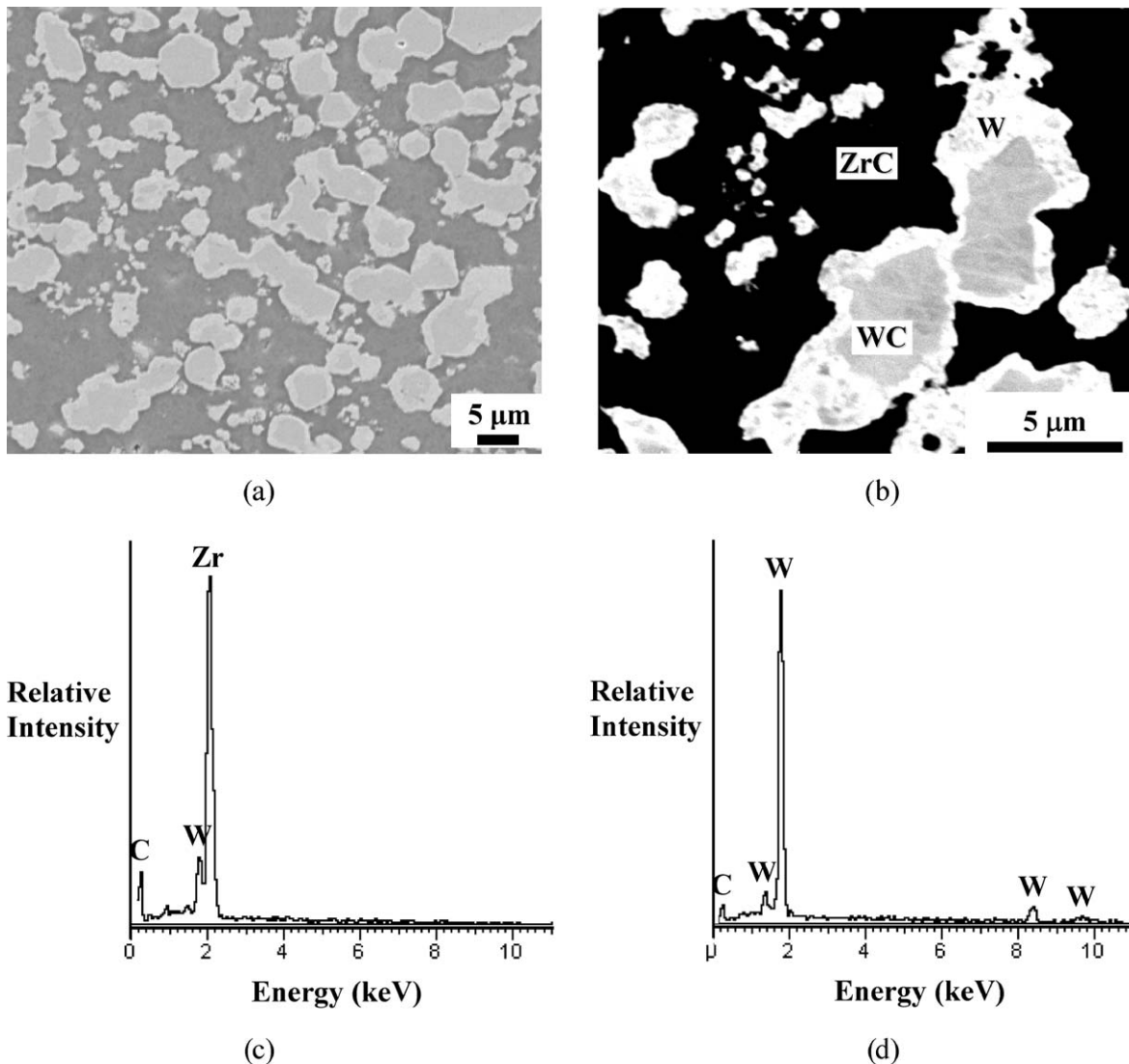
Figure 1 (a) Secondary electron and (b) backscattered electron images of a composite specimen generated by the reactive infiltration of \text{Zr}_2\text{Cu}(\text{l}) into a porous WC preform (43.5 vol% porosity) at 1300^\circ\text{C} for 8 h. EDX patterns obtained from the dark matrix phase and the grey core of the particles in (b) are shown in (c) and (d), respectively. (e) Backscattered electron image of a composite specimen generated by the reactive infiltration of \text{Zr}_2\text{Cu}(\text{l}) into porous WC preform (42.4 vol% porosity) at 1300^\circ\text{C} for 0.5 h. (f) XRD patterns obtained from WC preforms ( 46 \pm 1\% porosity) after infiltration and reaction with \text{Zr}_2\text{Cu}(\text{l}) for 0.5, 2, 4 and 8 h. (g) EDX pattern obtained from an isolated region containing a Cu-rich phase.
