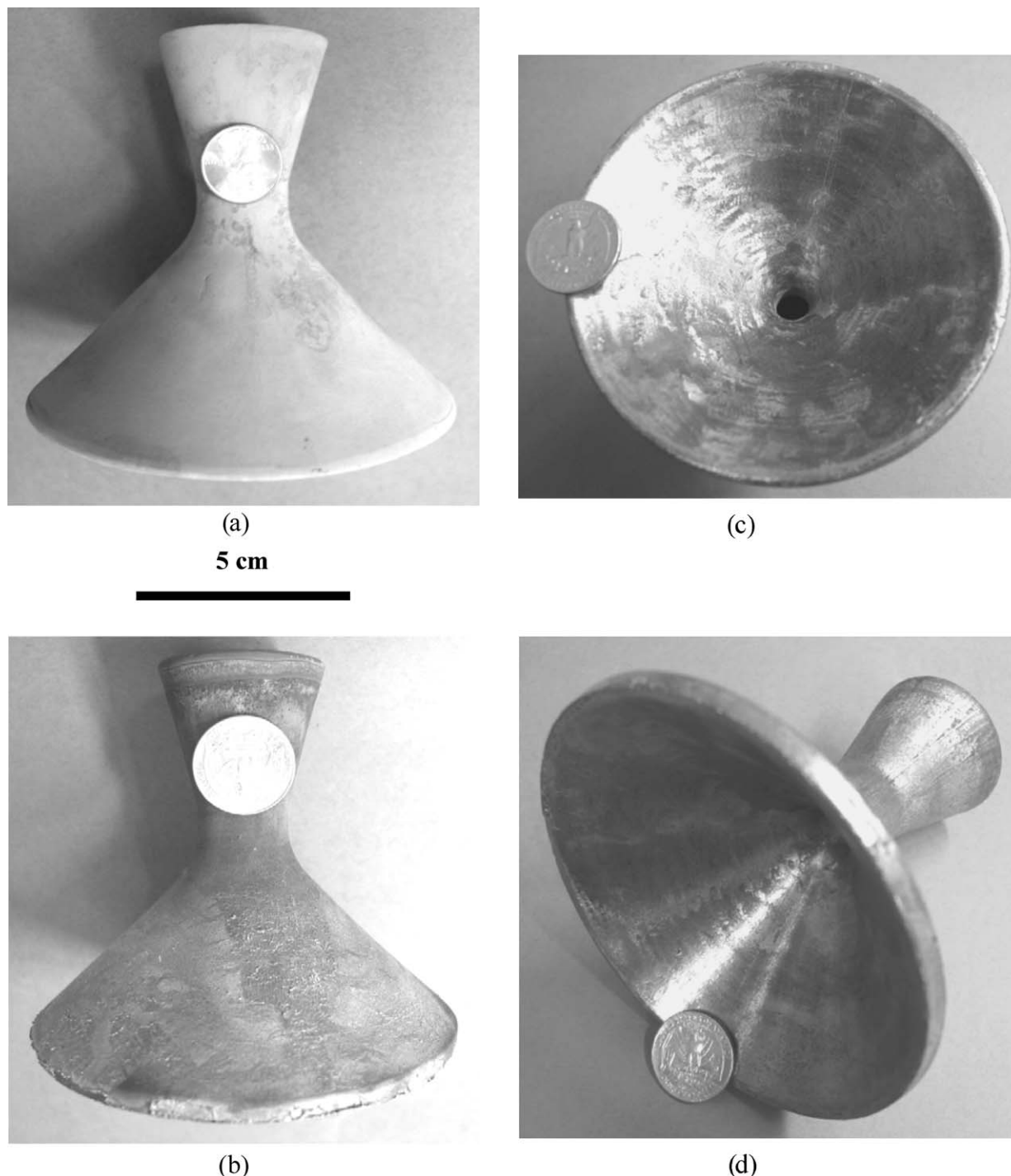
Figure 3 Optical photographs of (a) a nozzle-shaped WC preform (52.0 vol% porosity), and (b) the same specimen after reactive infiltration with Zr 2 Cu(l) (immersion for 10 min at 1200°C, followed by heating at 2°C/min to 1300°C), and (c), (d) after removal of the excess solidified metal on the nozzle surfaces by polishing.
